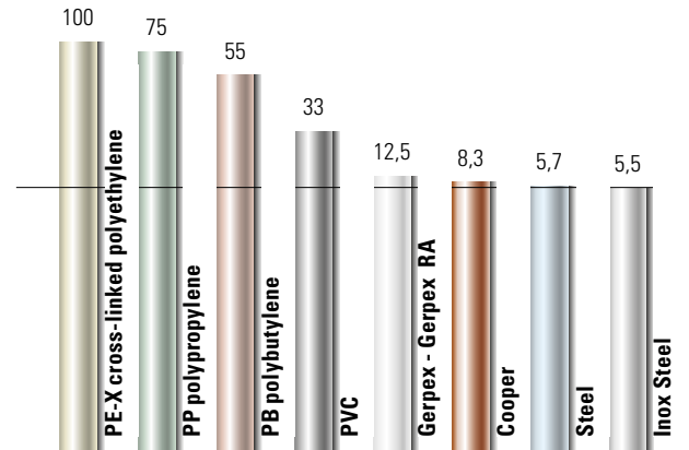
linear thermal expansion for 10 m pipes of different materials \Delta T 50^\circ\text{C} (values expressed in mm)
